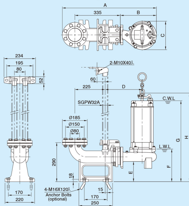
TOS-80-SV(3") - For 2 ~ 5HP SV Pump
