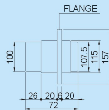
External Connector
