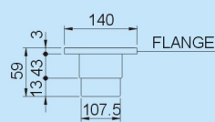
Inlet Collar
